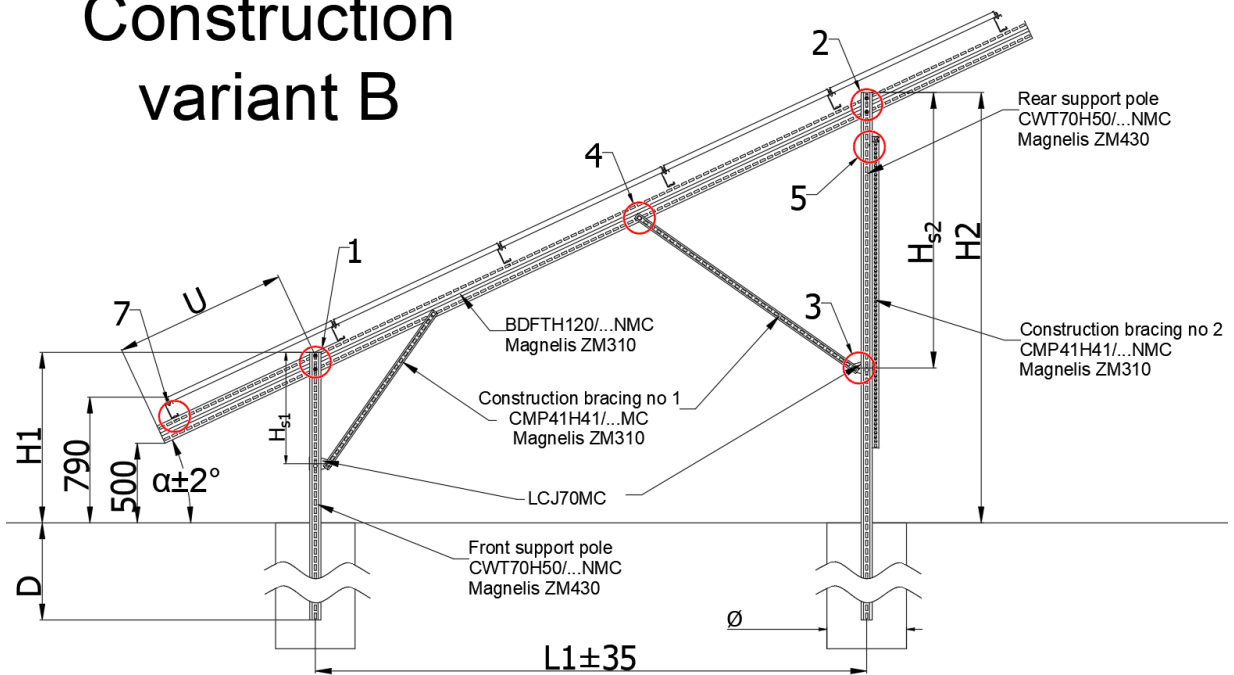
Fig. 1 Side view of the structure
